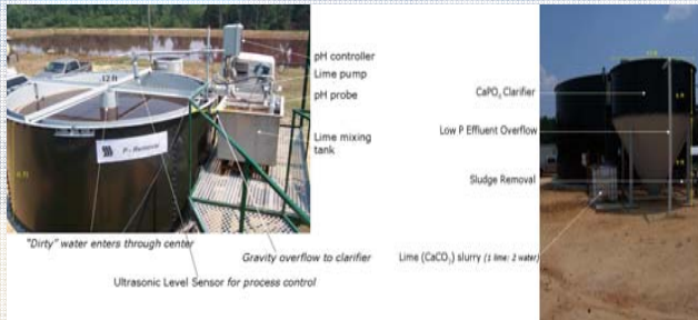
Total Phosphorus Removal of Separated Parlor Wastewater: Idaho
